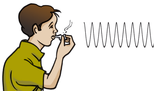
Fig. 10.18 : Frequency determines the pitch of a sound
