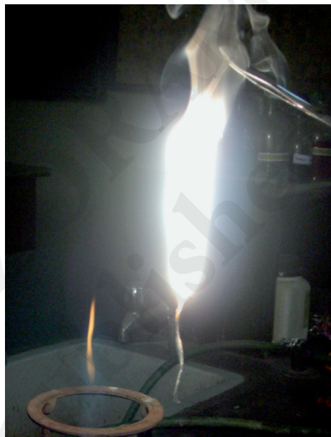
Fig. 4.1 : Burning of magnesium
