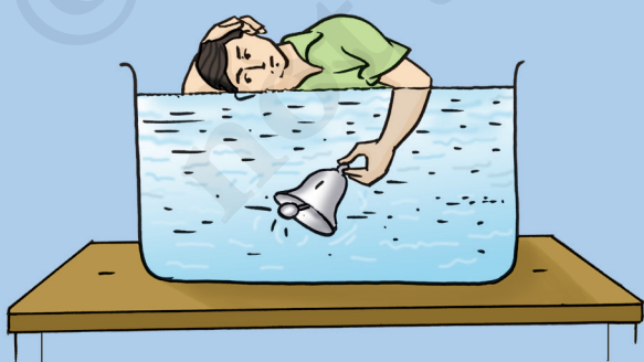
Fig. 10.11 : Sound travelling through water
