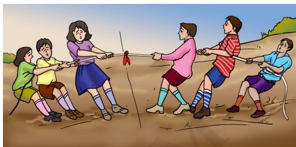
Fig. 8.5 : The rope may not move if the two teams pull at it with equal force
