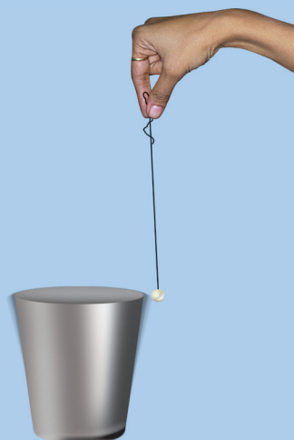
Fig. 10.17 : Thermocol ball touching the vibrating glass tumbler
